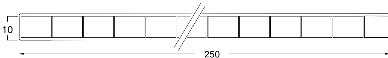
KA 150.11
