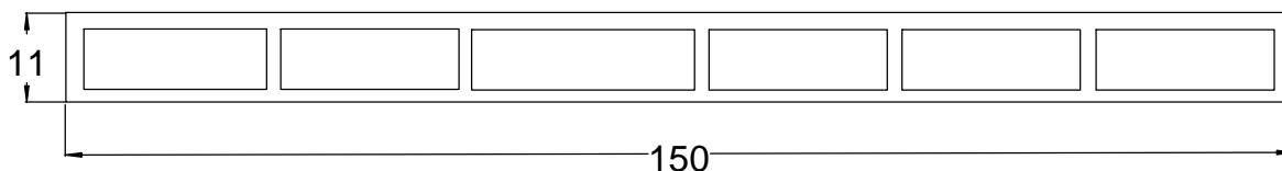
KA 150.11
